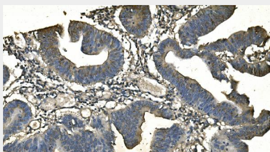
Figure 2. IHC analysis of CD13/ANPEP using anti-CD13/ANPEP antibody (M02591-4).
